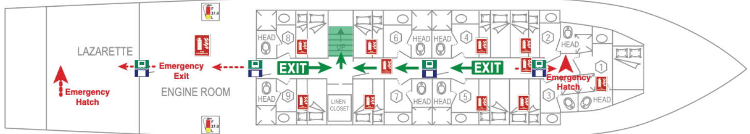
LOWER DECK
